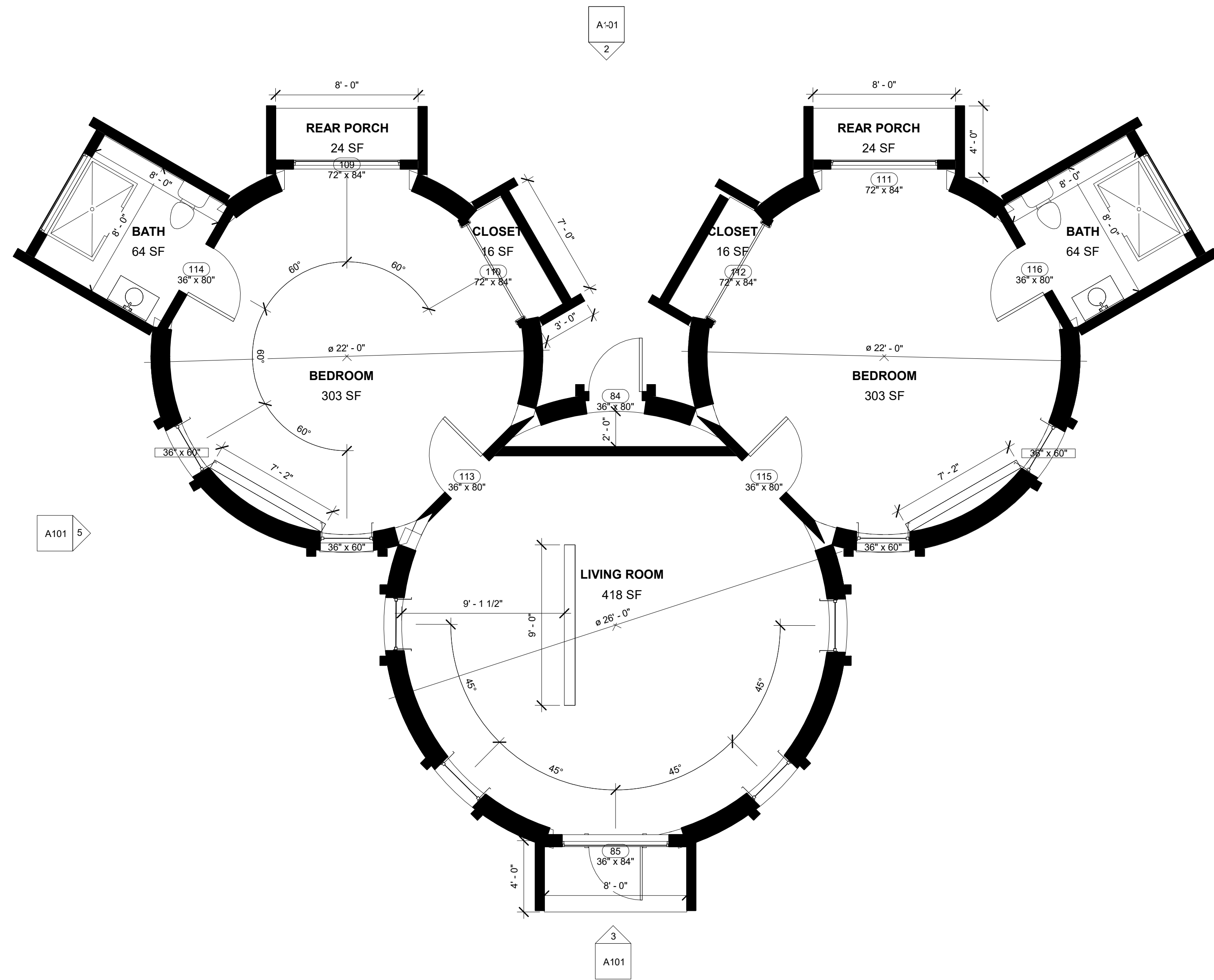
GROUND LEVEL - 2 BEDROOM DIMENSION PLAN 1/4" = 1'-0"
